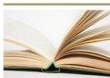
Superconductivity and Magnetism in Iron Arsenides and Cuprates
