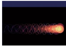
Self-focusing of electromagnetic wave in collisional plasma
